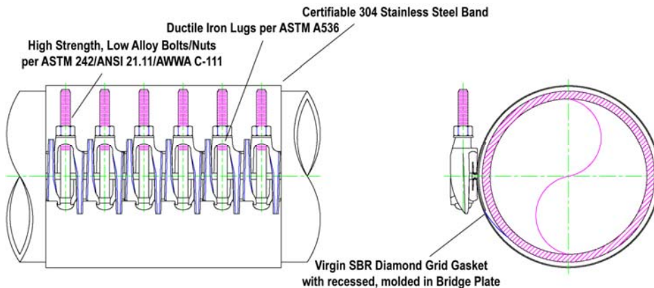
JCM 101 Universal Clamp Coupling Image reflects 18" width
