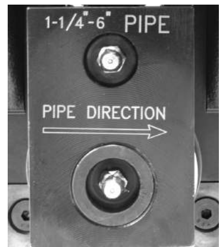
Figure 4. Pipe Direction on Slide Block
